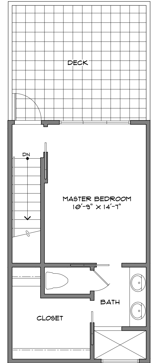
THIRD FLOOR 384 SF DECK 188 SF
