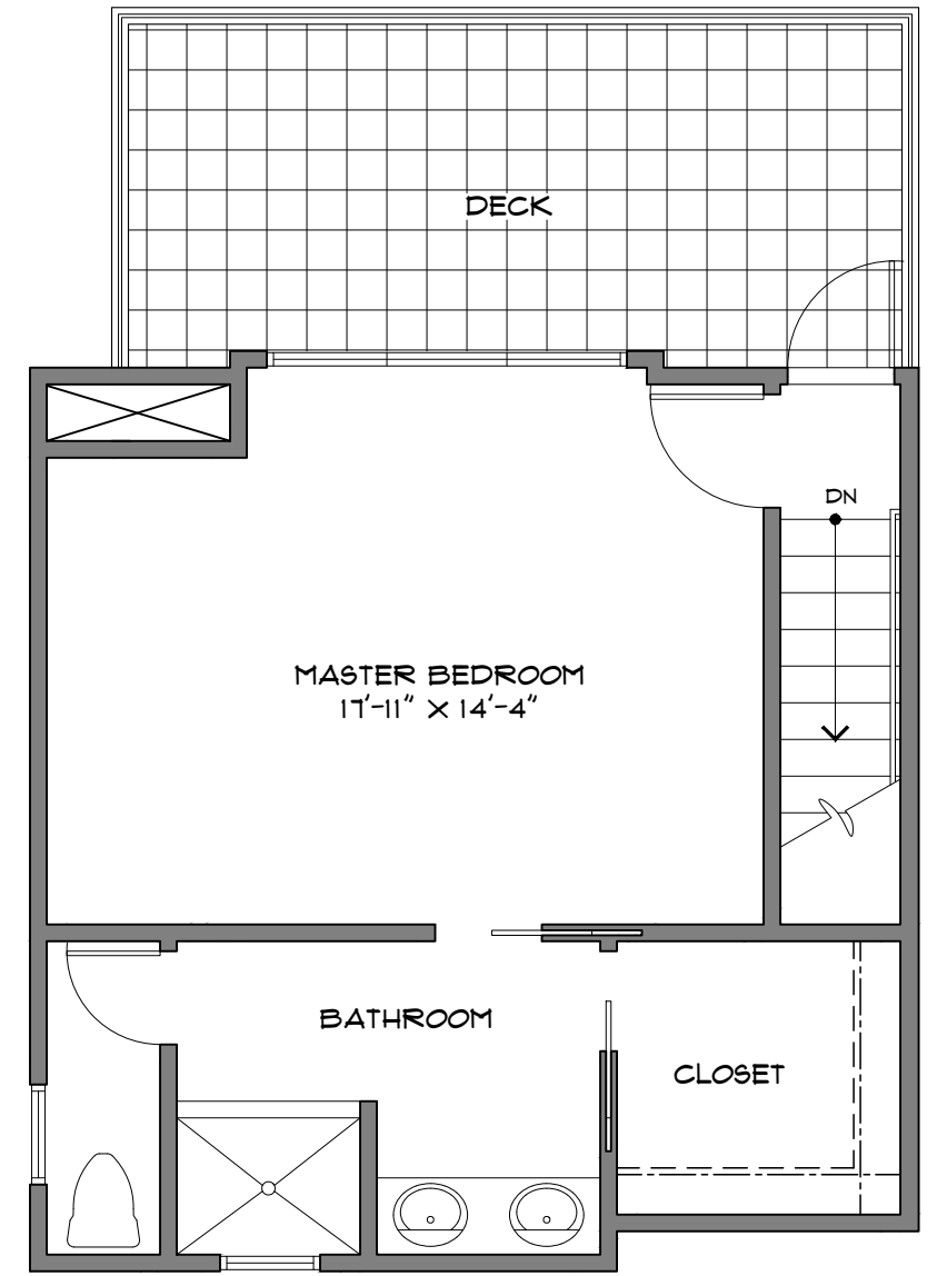
THIRD FLOOR 498 SF
