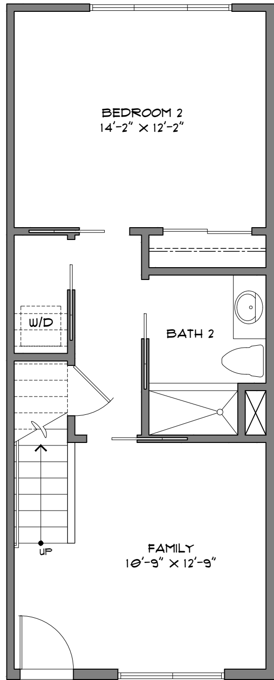
FIRST FLOOR 575 SF
