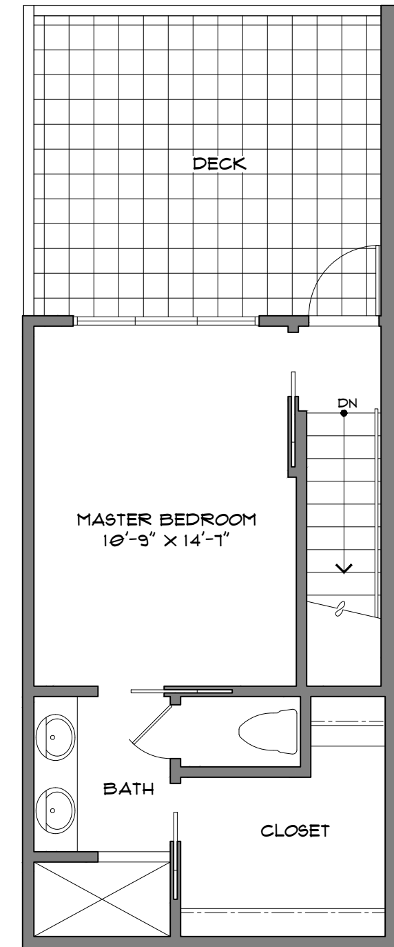
THIRD FLOOR 384 SF DECK 189 SF
