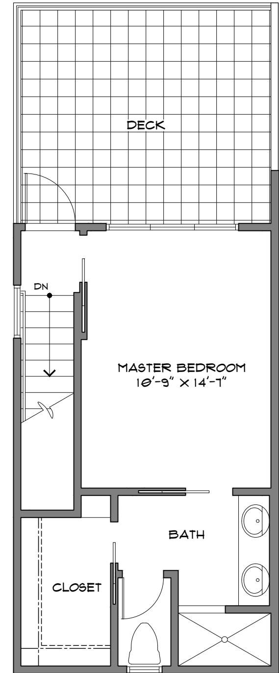
THIRD FLOOR 384 SF
