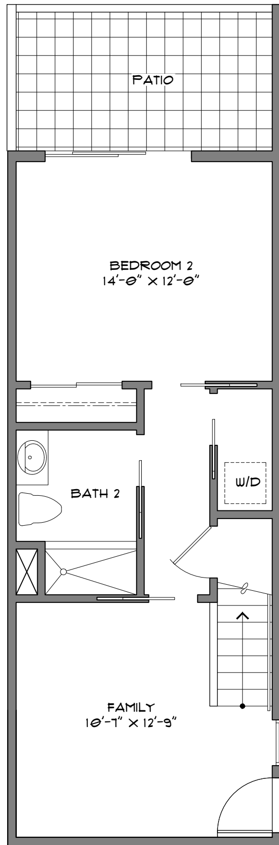
FIRST FLOOR 512 SF PATIO 121 SF
