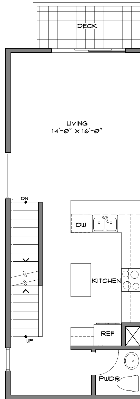
SECOND FLOOR 572 SF
