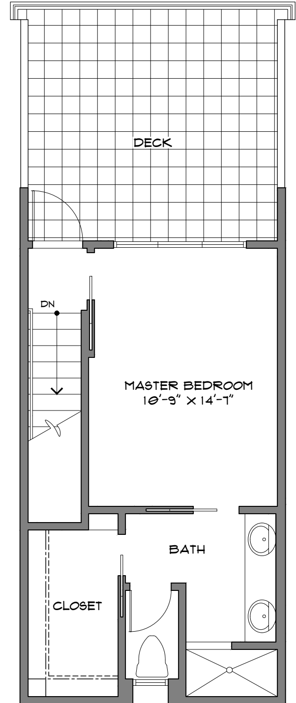
THIRD FLOOR 392 SF
