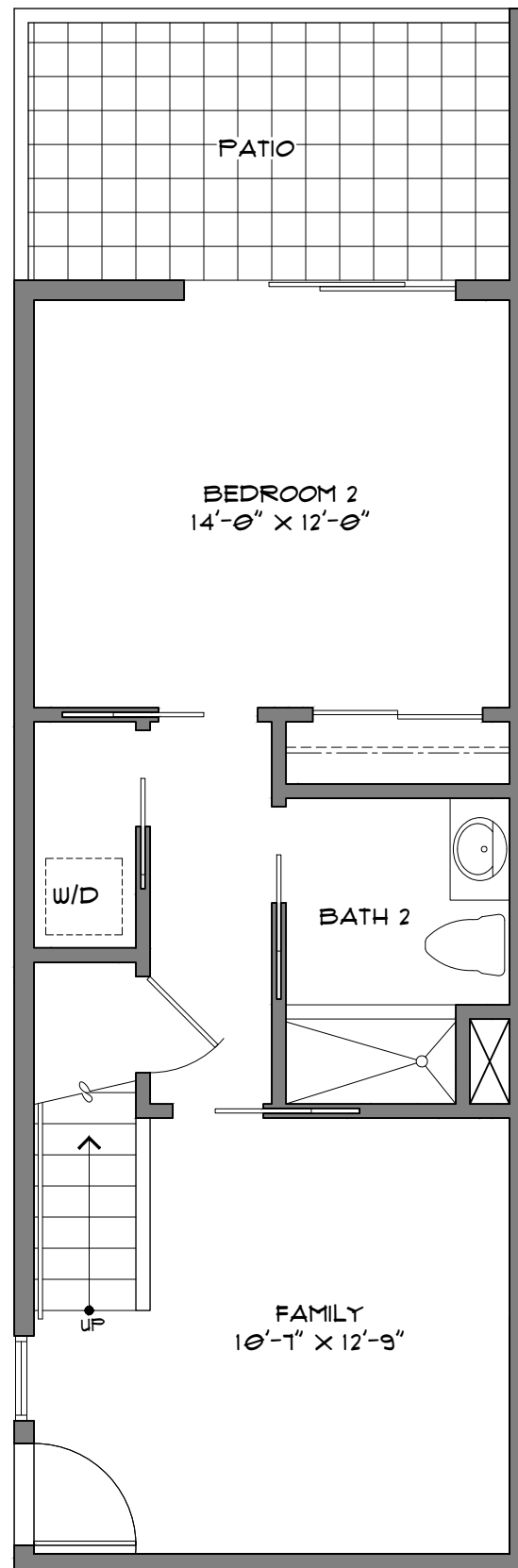
FIRST FLOOR 572 SF
